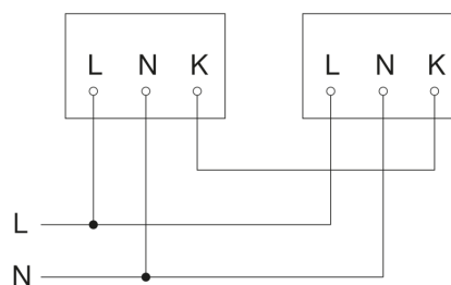
Master/master interconnection circuit diagram
